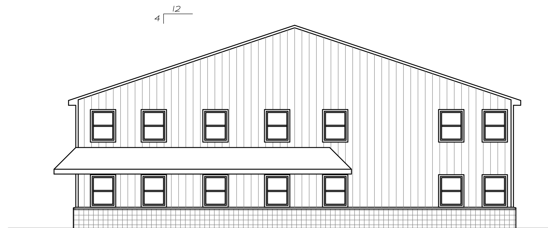
2 North Elevation 1/8"=1'-0"
