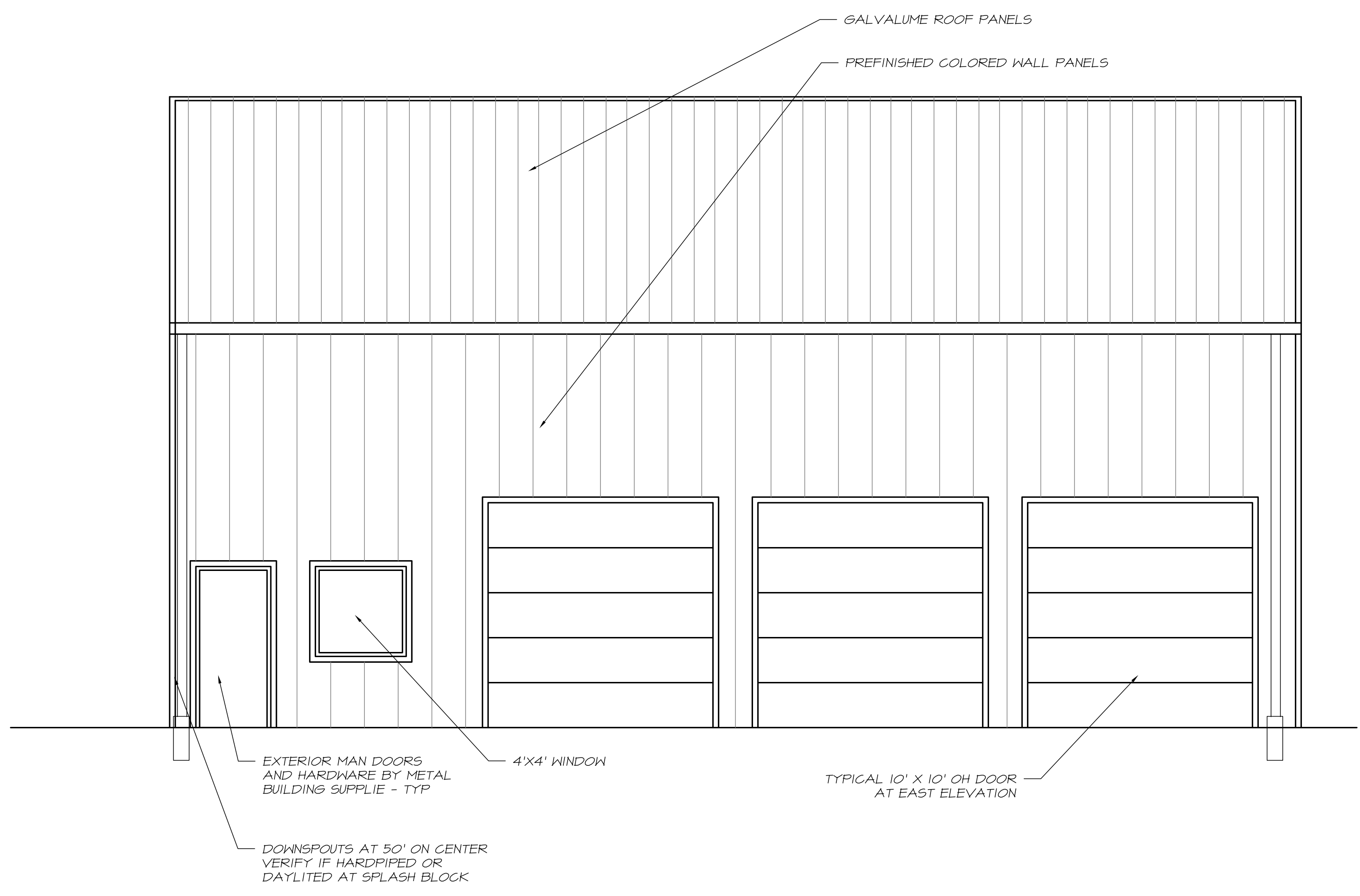
2 East Elevation 1/8"=1'-0"
