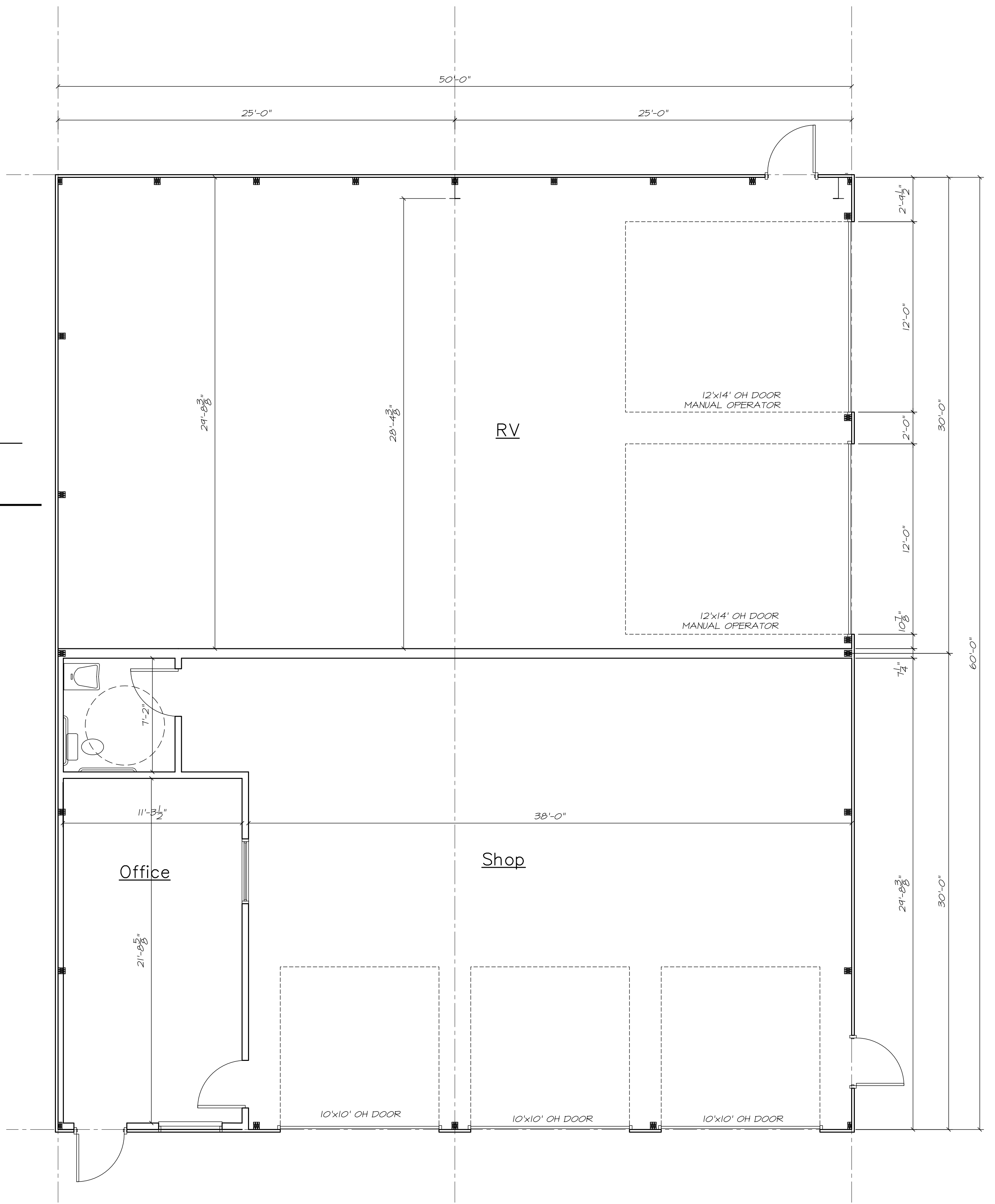
Proposed Floor Plan 1/4"=1'-0"
