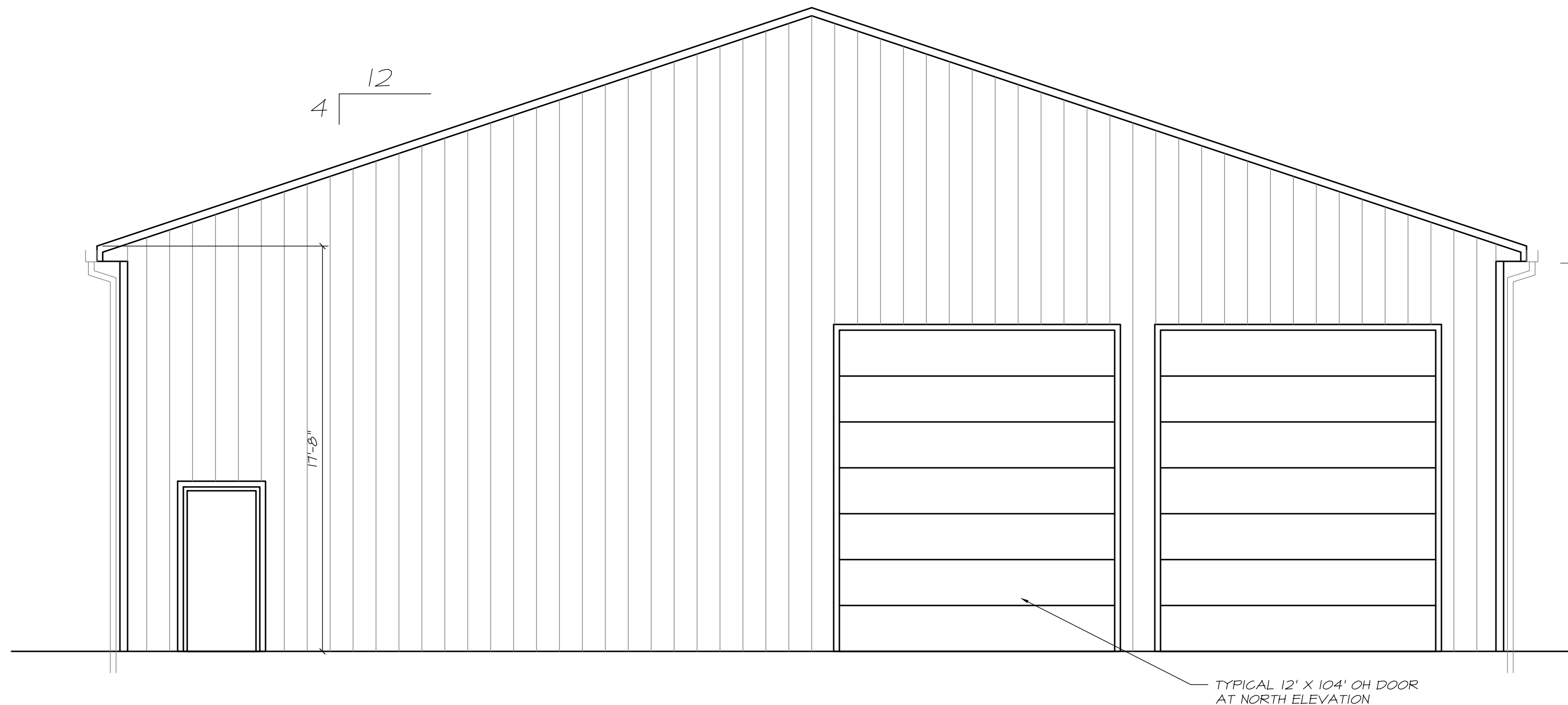
1 North Elevation 1/8"=1'-0"
