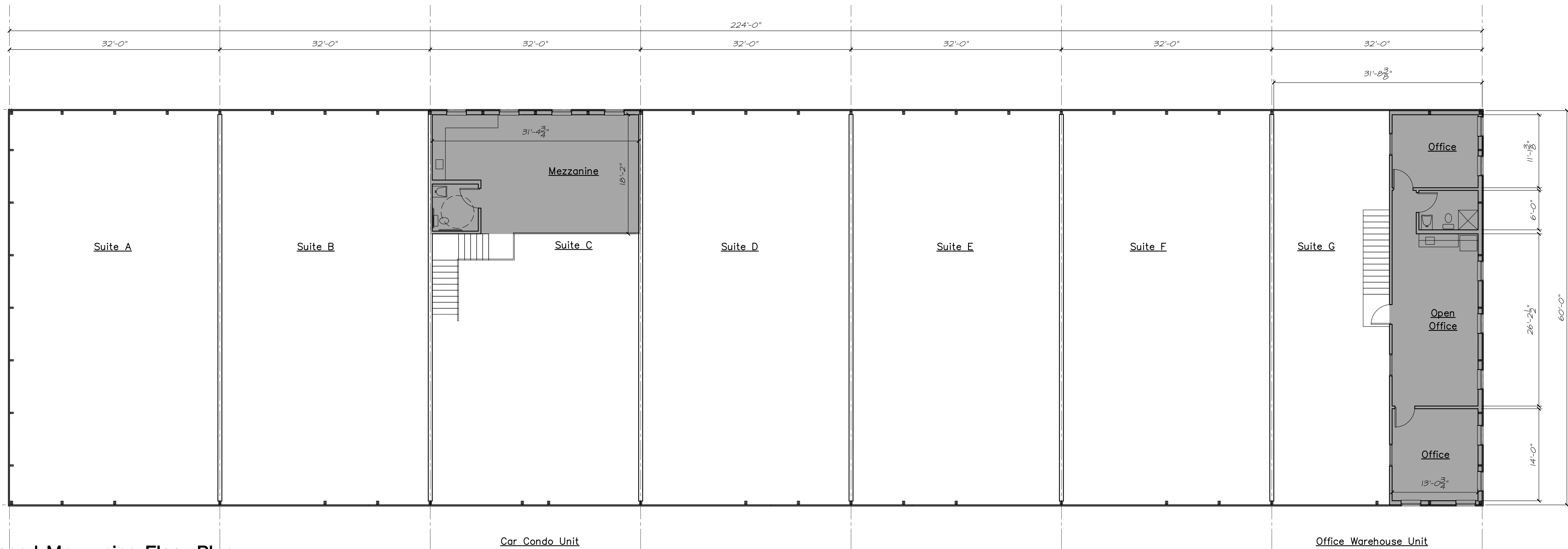
Proposed Mezzanine Floor Plan 1/8"=1'-0"
