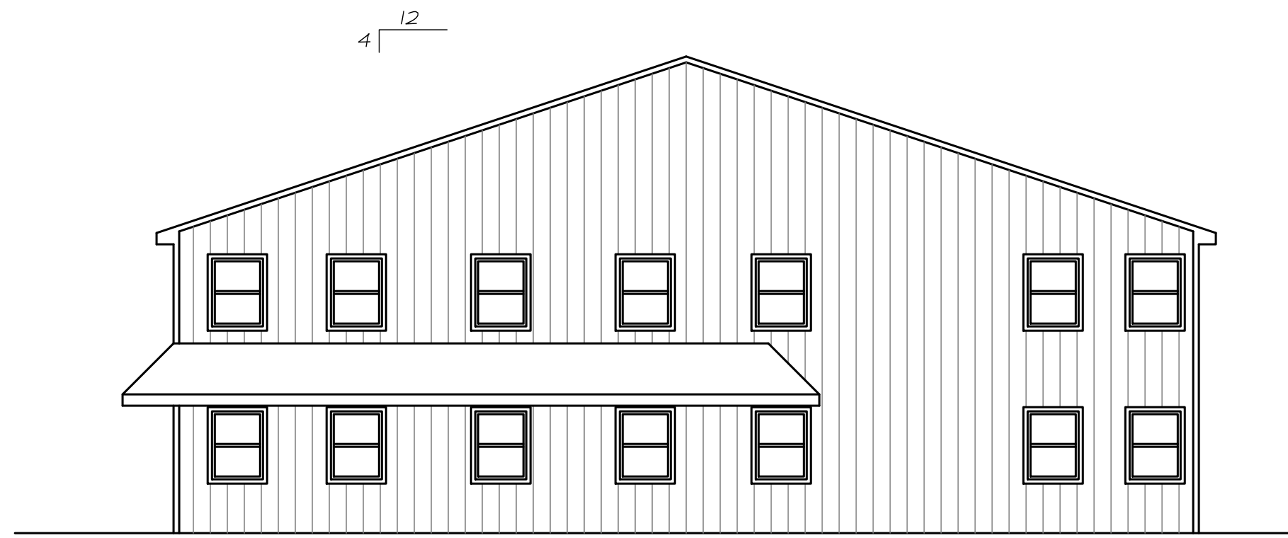
2 North Elevation 1/8"=1'-0"
