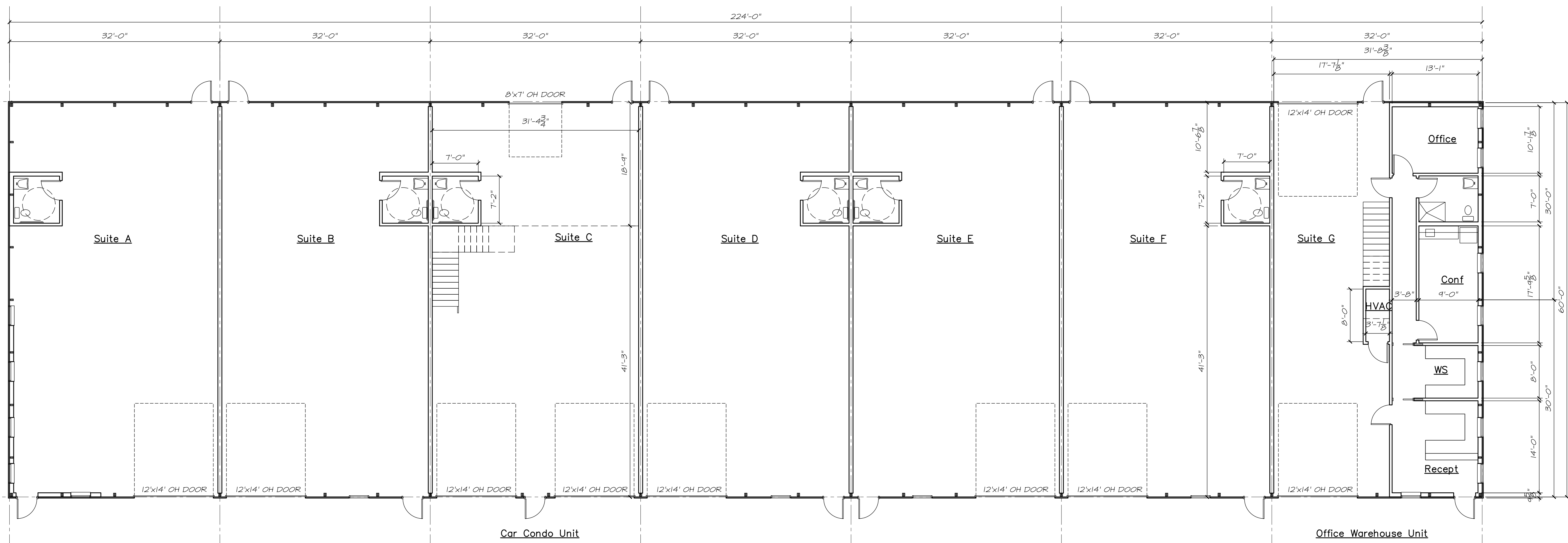
Proposed First Floor Plan 1/8"=1'-0"
